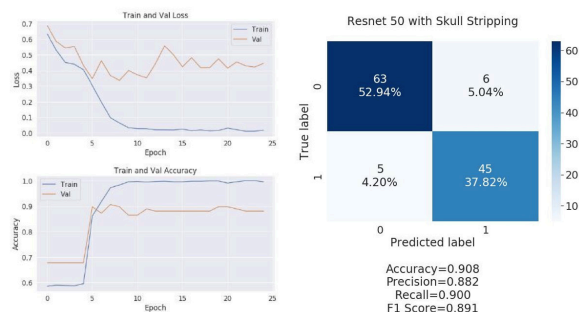
Figure 15: Results for ResNet50 with skull stripping preprocessing.
