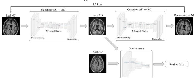
Figure 6: CycleGAN Architecture.
