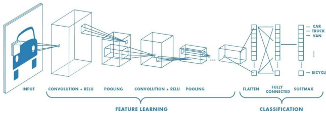
Figure 1: CNN Architecture. Adapted from Buetti-Dinh et al. 4
