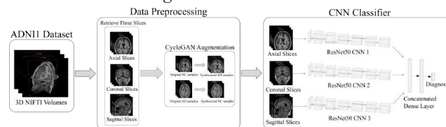
Figure 5: Overview of the model pipeline.
