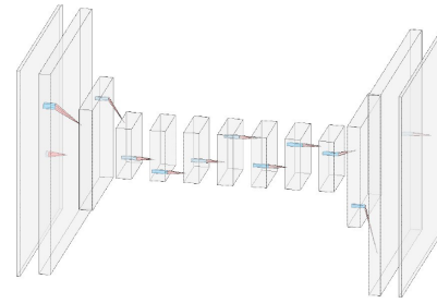
Figure 7: CycleGAN Generator Architecture.
