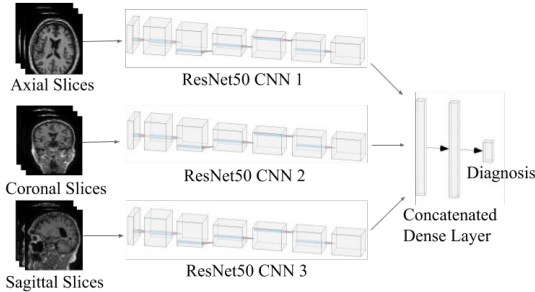
Figure 10: Proposed Multiple CNN architecture.
