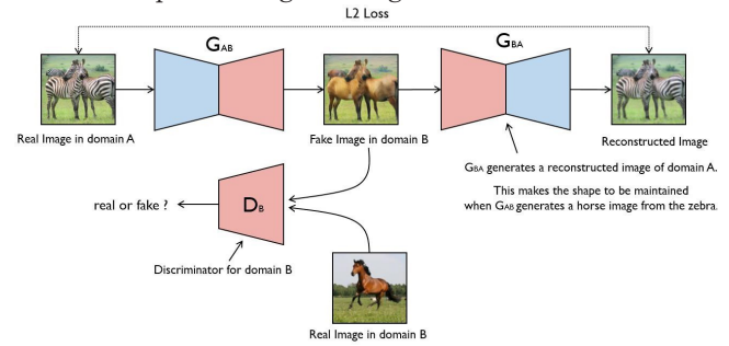
Figure 3: CycleGAN architecture. Adapted from Goodfellow et al. 8
