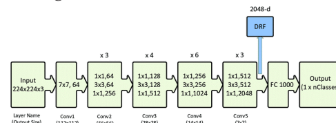
Figure 9: ResNet50 Architecture. Adapted from. 20
