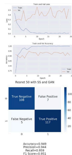
Figure 16: Results for ResNet50 with GAN data augmentation.
