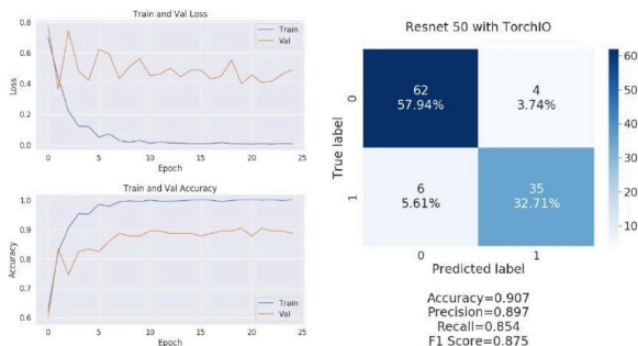
Figure 14: Results for ResNet50 with TorchIO preprocessing.
