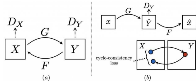
Figure 4: CycleGAN Loss. Adapted from Hosseini-Asl 9
