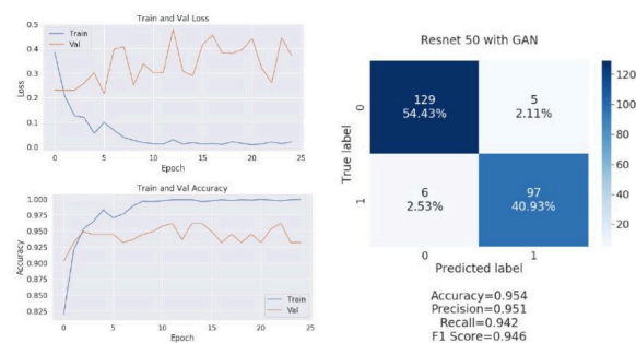
Figure 16: Results for ResNet50 with GAN data augmentation.
