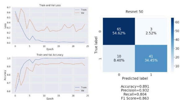
Figure 13: Results for ResNet50.
